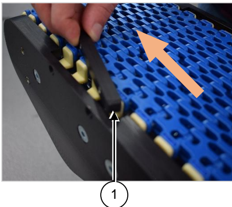
Fig. 3: Assembling the modular chain belt
