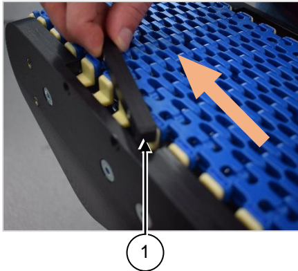
Fig. 4: Adjust modular belt chain
