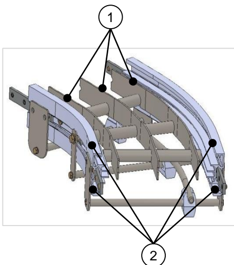
Fig. 2: Assembly the slide rails and slide profiles on the modular belt conveyor
