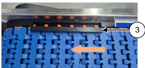
Fig. 3: Assembling the modular chain belt
