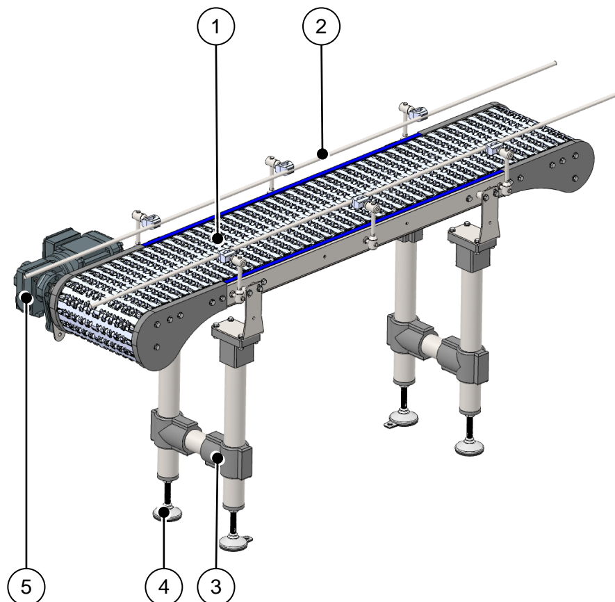
Fig. 1: Overview of MB-flex O stainless steel (example)
